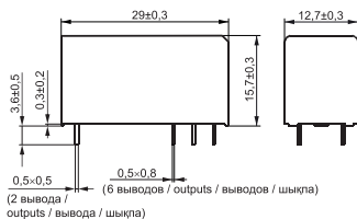
б) / b) IMR-470-ML-2-REL-A220-N00; IMR-470-ML-2-REL-D024-N00
