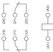
б) / b) IMR-470-ML-2-REL-A220-N00; IMR-470-ML-2-REL-D024-N00
