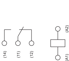
а) IMR-470-ML-1-REL-A220-N00; IMR-470-ML-1-REL-D024-N00
