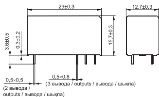
а) IMR-470-ML-1-REL-A220-N00; IMR-470-ML-1-REL-D024-N00
