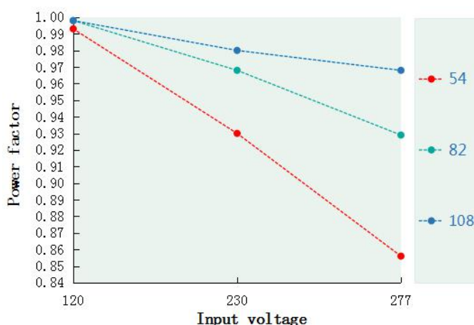
Power factor VS Input voltage(DL-75W-V108A/P/X-MXG)
