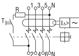
Figure 4 – Electric schematic diagram of four-polar VDs
