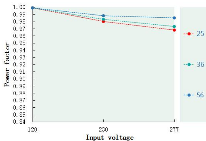
Power factor VS Input voltage(DL-200W-V56A/P/X-MXG)
