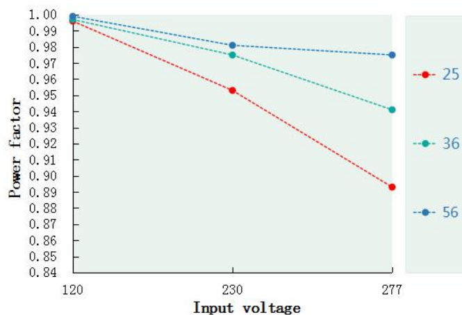
Power factor VS Input voltage(DL-100W-V56A/P/X-MXG)
