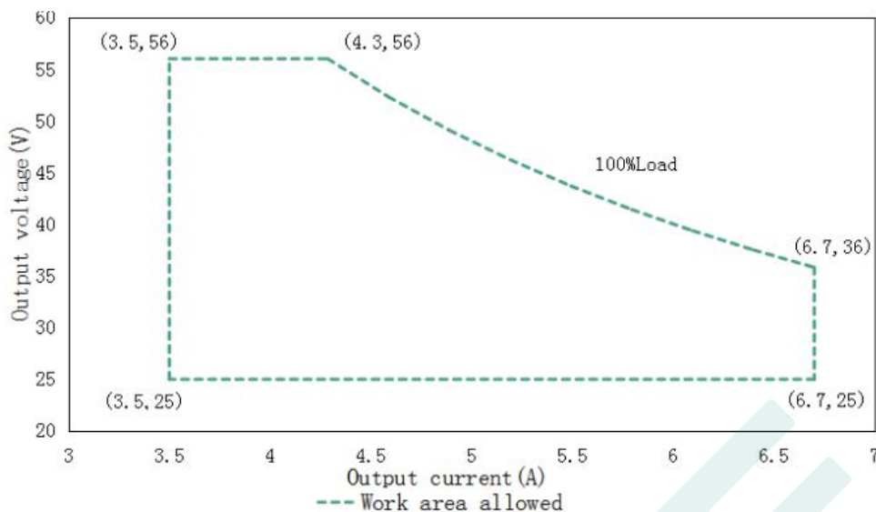
Output voltage VS Output current of DL-240W-V56A/P/X-MXG (input: 120-277Vac)
