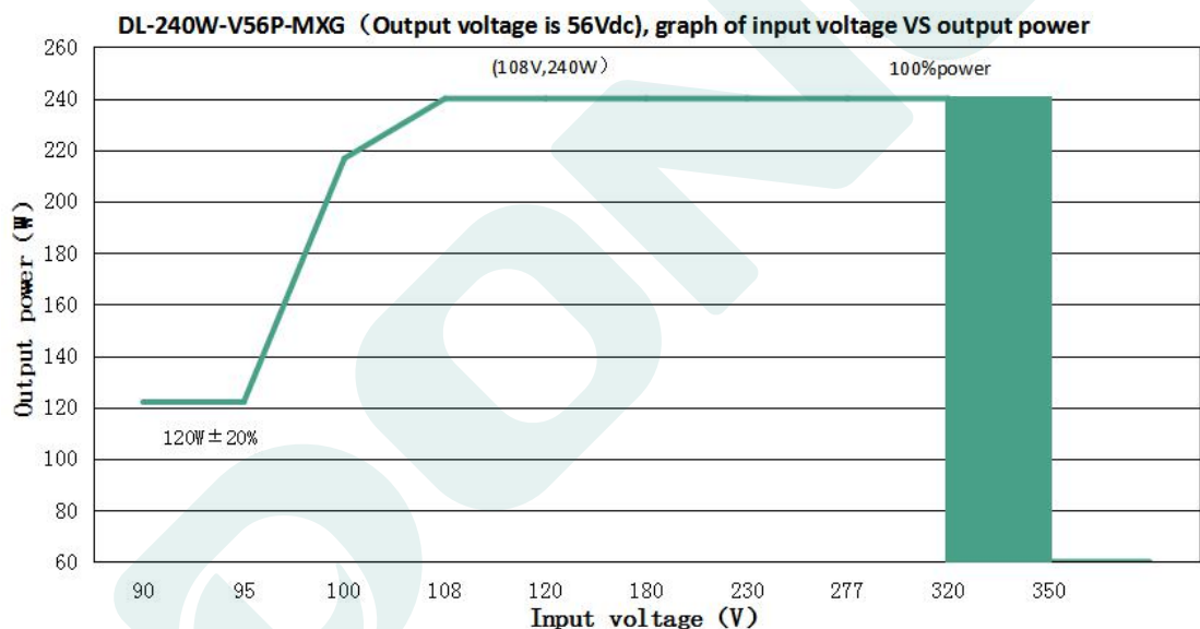
DL-240W-V56A/P/X-MXG (When the output voltage is 56Vdc, the rated output current value and output power corresponding to different input voltage)
