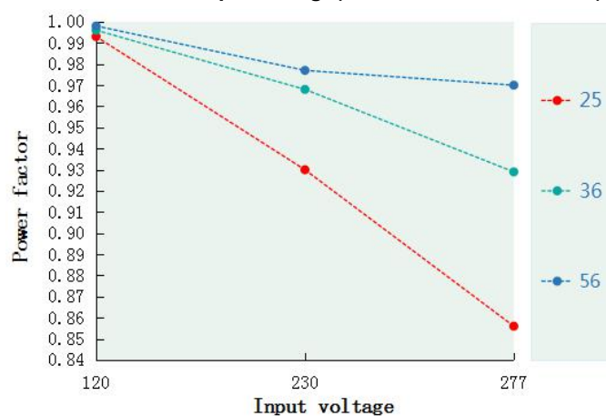
Power factor VS Input voltage(DL-150W-V56A/P/X-MXG)
